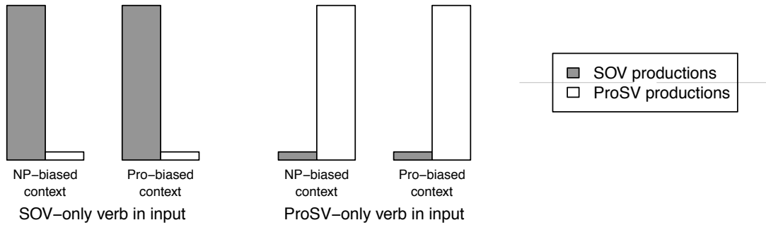
Figure 3a: Hypothetical proportions of SOV and ProSV productions predicted by lexical conservatism in which productions depend only on whether verbs were SOV or ProSV in the input.
